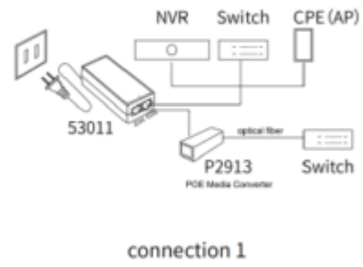
PoE Power adapter connection diagram
